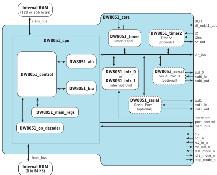
Figure 3. DW8051_core
