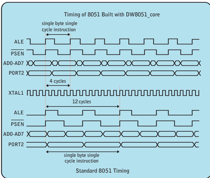
Figure 4. Instruction cycle timing comparison
