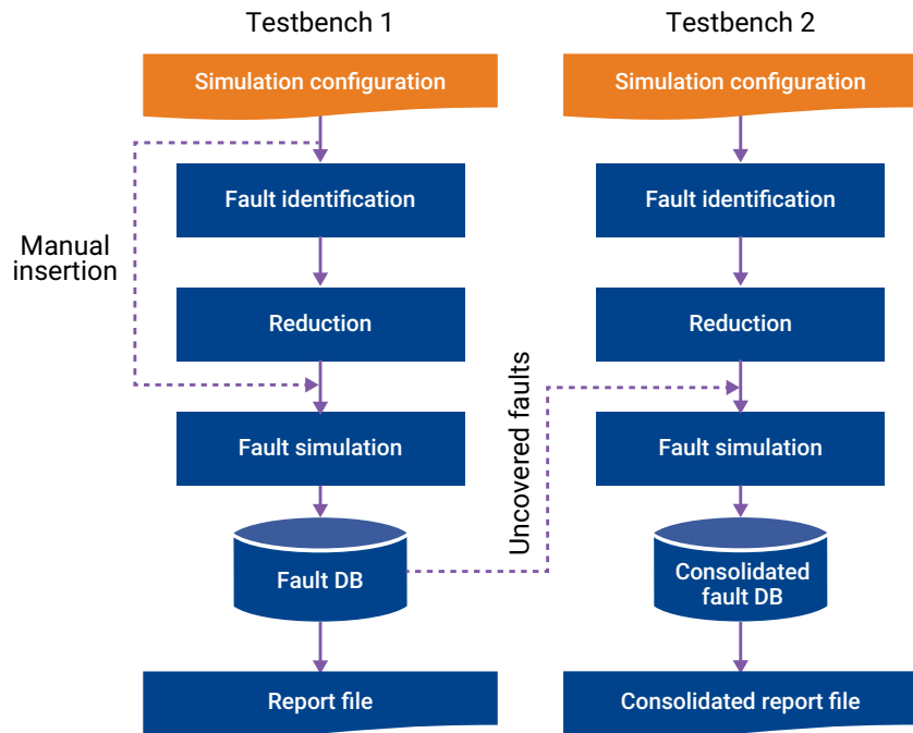
Figure 9: Multi-testbench Flow
