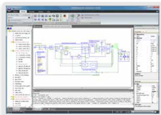
Figure 1: Hybrid Vehicle Powertrain design
