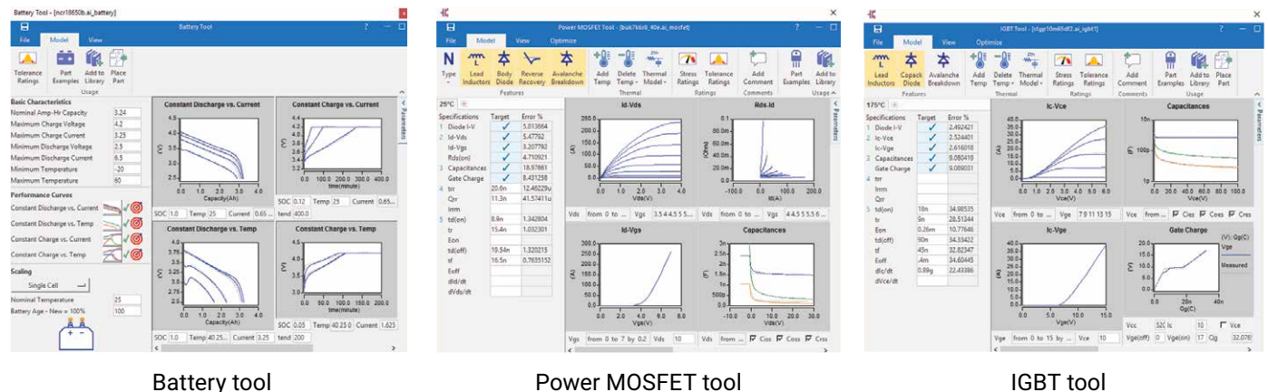
Figure 3: Battery, Power MOSFET and IGBT characterization tools in Saber
