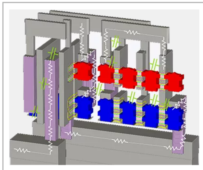
Figure 9: Interconnect structures with Rafael FX
