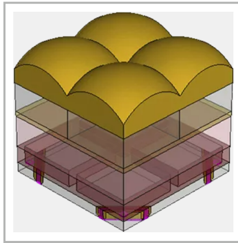
Figure 6: CIS device created with Sentaurus Structure Editor
