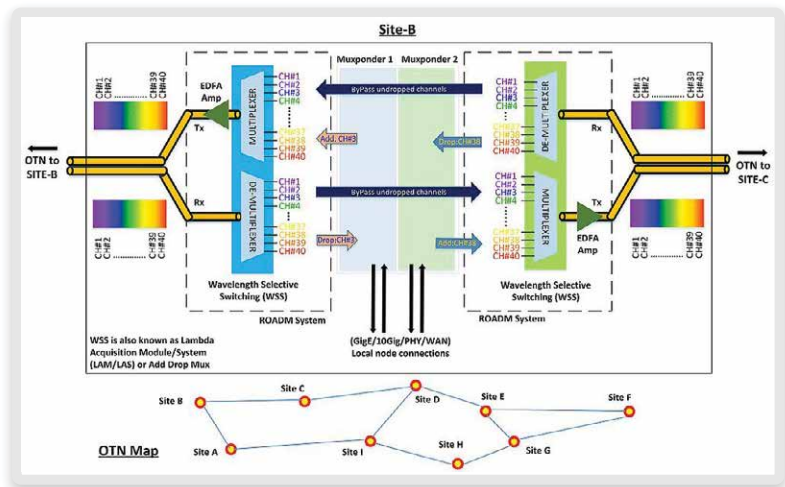
Figure 1. Functional details of a ROADM at an optical transport network (OTN) node
