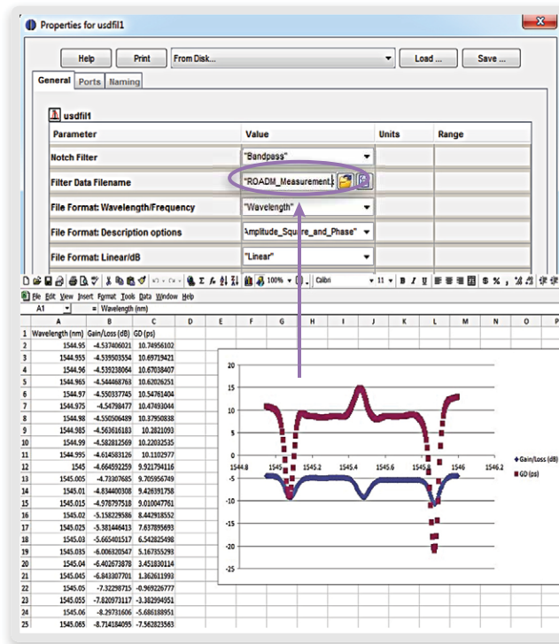
Figure 2. Using ROADM measurement data (lower) to model it in OptSim (upper)
