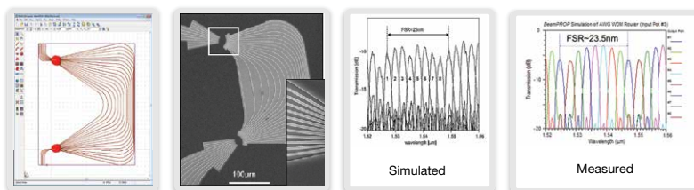
Figure 1. The BeamPROP simulation of IMEC's AWG correlated closely with measured results. Source: Bogaerts, et.al., JSTQE,12,6,pp1394 (2006)
