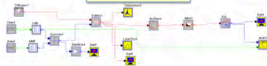
MZM Link Jitter and Noise Free
