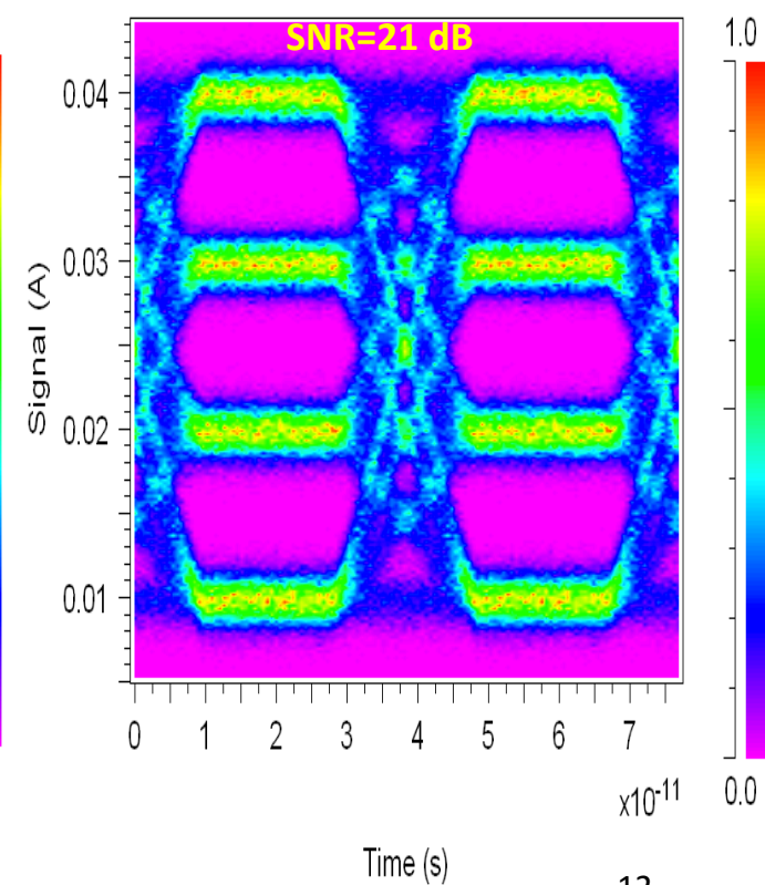
DML Driver with Noise and Jitter
