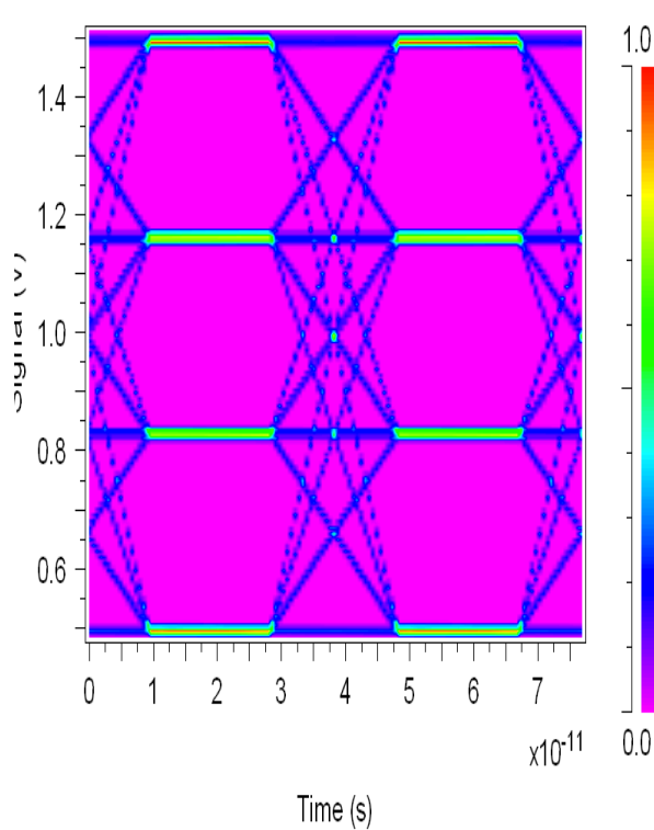
MZM Driver without Noise and Jitter
