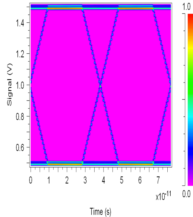
MZM Driver Output
