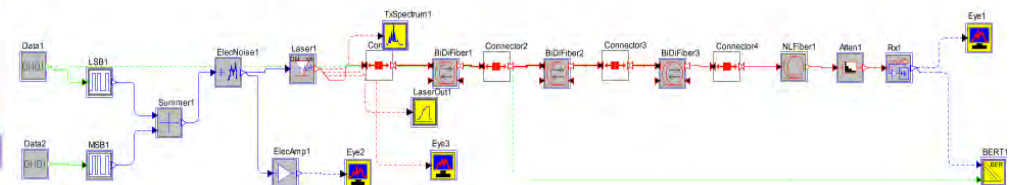
DML Link with Jitter, Noise, MPI*
