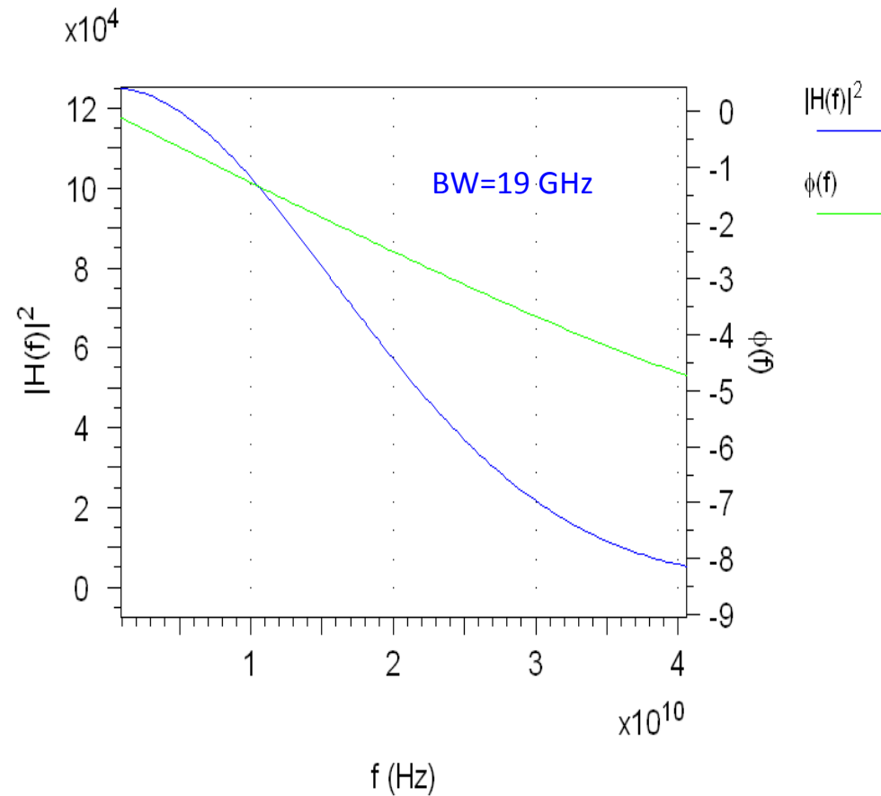
Receiver cumulative response
