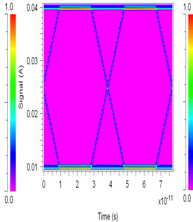
DML Driver Output
