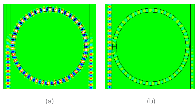
Figure 1: Field distribution in the SOI based Ring Resonator (a) at resonance and (b) off resonance
