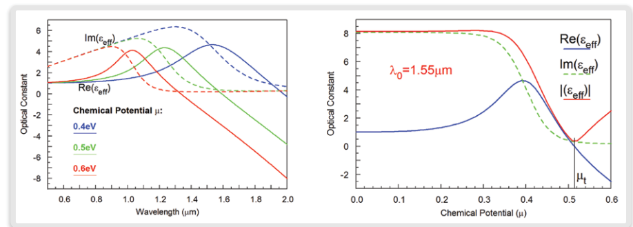
Figure 1. Graphene optical constant versus wavelength and chemical potentials computed in the RSoft tools
