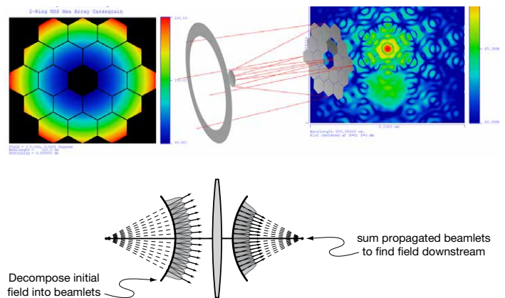
Figure 6: Beam Synthesis Propagation's beamlet-based wave propagation algorithm performs beam propagation analysis more accurately and efficiently than any other commercially available tool.
