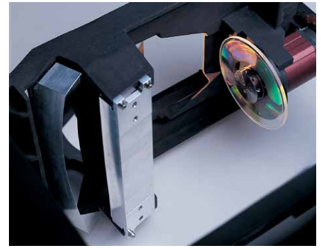
Holographic scanner designed by our engineers and produced by Holographix for high quality, large format color printing
