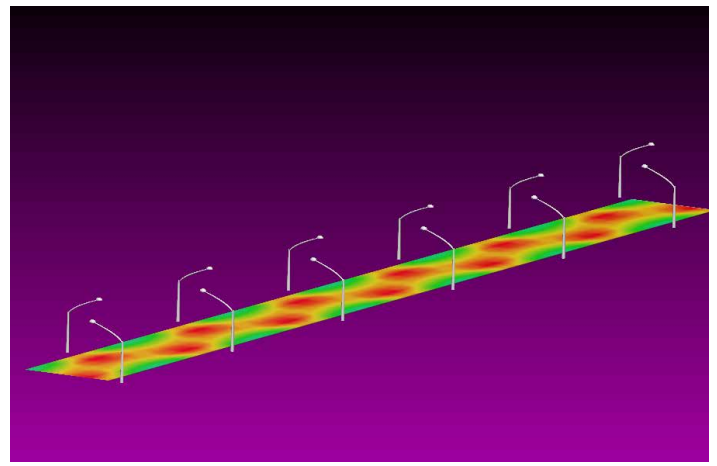
LED street lighting design and analysis completed in LightTools
