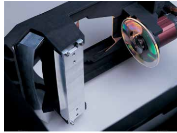
Holographic scanner designed by our engineers and produced by Holographix for high quality, large format color printing
