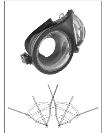
Wide-field, unity magnification dive mask designed by our engineers
