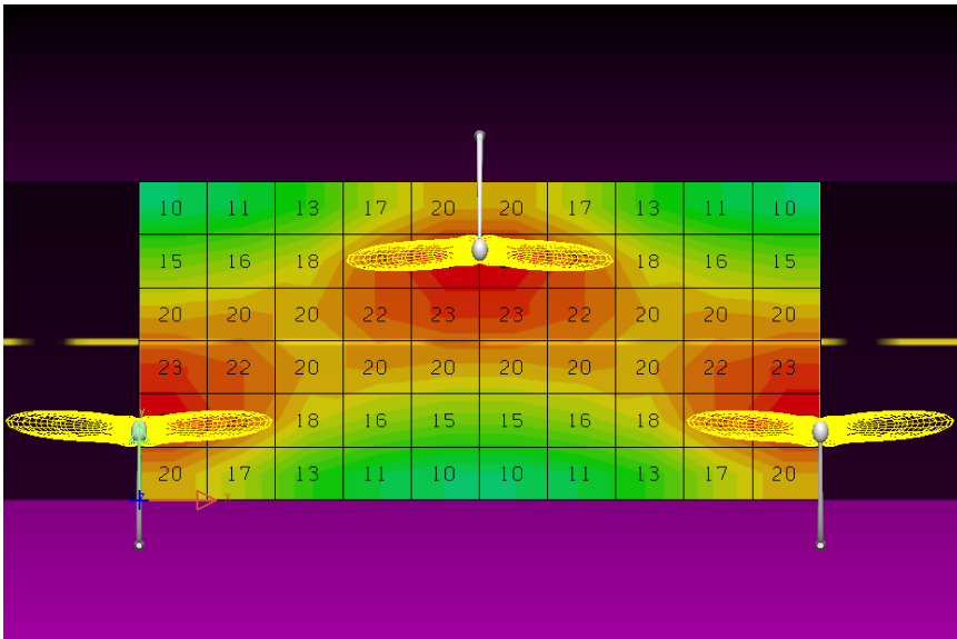
LED street lighting design and analysis completed in LightTools
