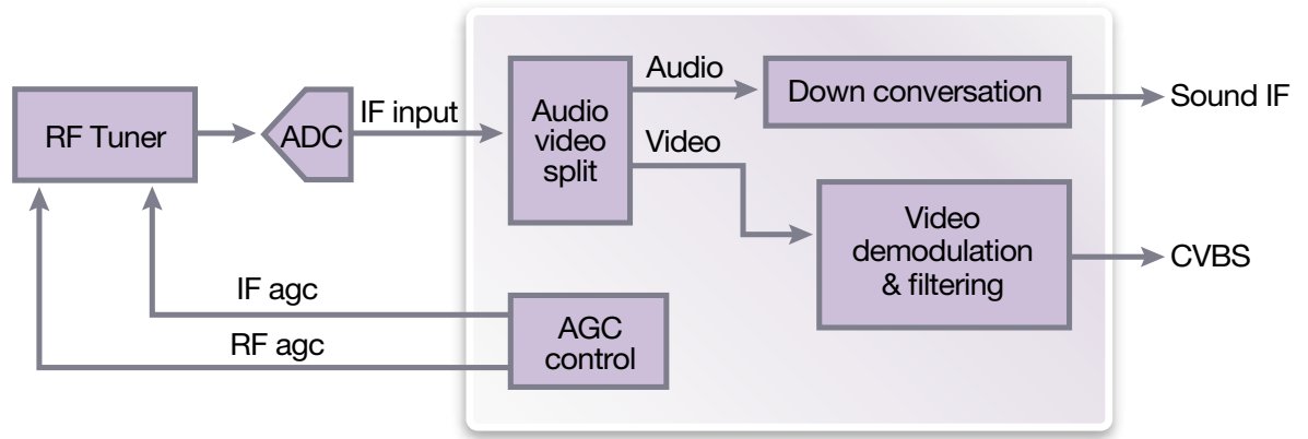
Figure 1: Digital Intermediate Frequency (DIF)
