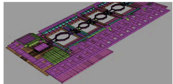
Figure 8. Low-noise amplifier (LNA) block meshed by Exalto
