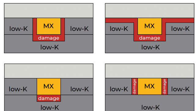
Figure 5. Types of dielectric damage
