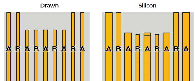
Figure 4. Multipatterning variation
