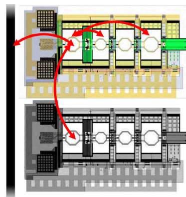
Figure 1. Various types of coupling that can be analyzed with Exalto, including stage-to-stage, block-to-seal ring, and block-to-block
