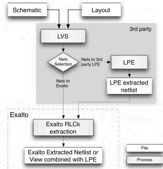
Figure 7. Integration of Exalto in the post-layout physical verification flow
