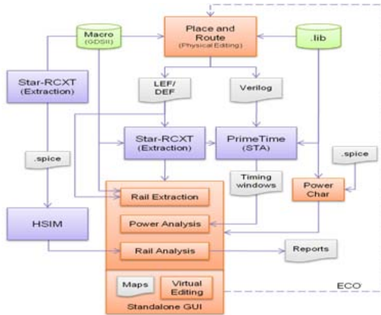
Figure 1: Bolted-On Rail Analysis Flow
