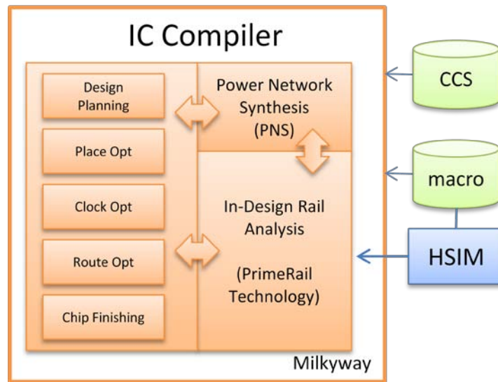
Figure 2: IC Compiler In-Design Rail Analysis with PrimeRail Technology
