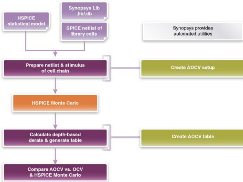
Figure 7: Depth-Based Derate Table Generation Process
