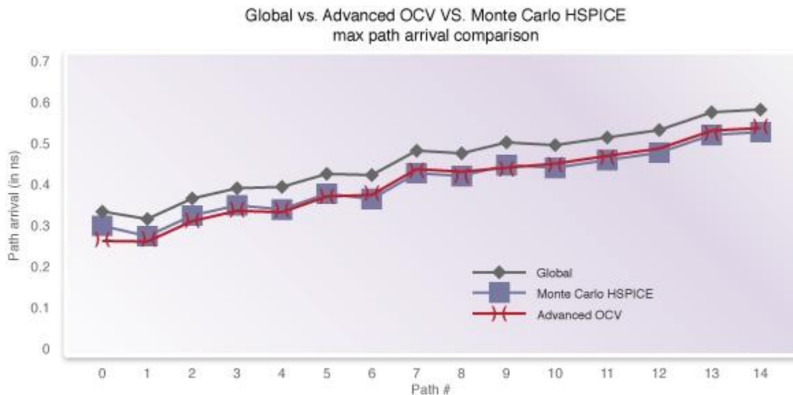
Figure 8: Advanced OCV Accuracy Results
