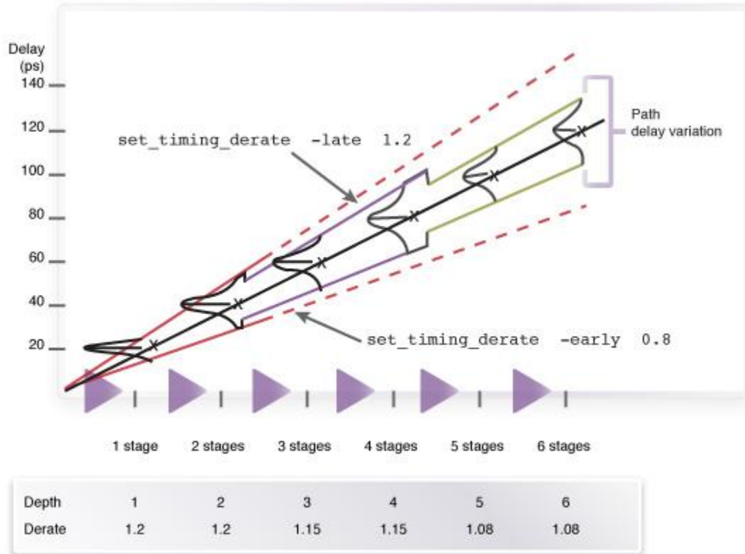
Figure 1: Depth-Based Statistical Analysis
