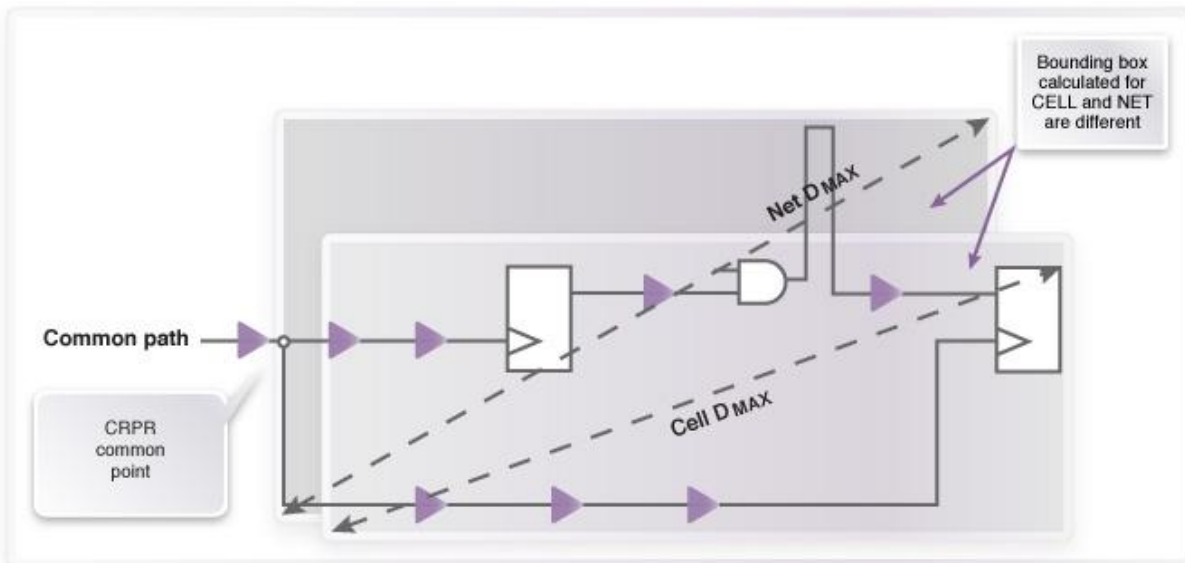
Figure 2b: Distance-Based Advanced OCV
