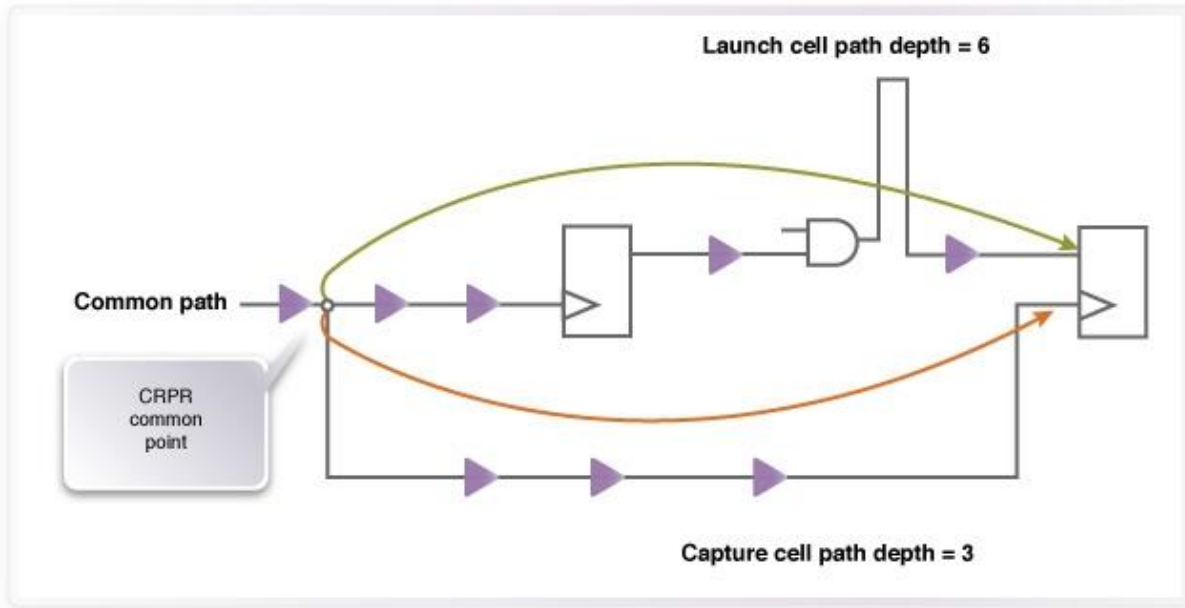
Figure 2a: Depth-Based Advanced OCV
