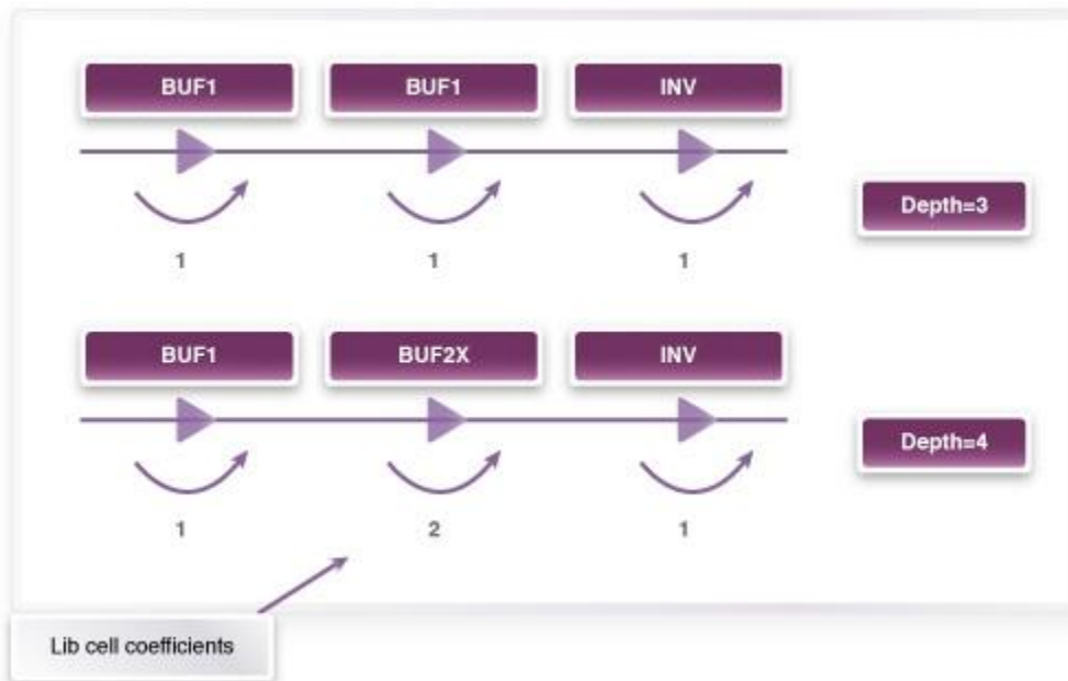
Figure 5: Cell-Based Depth Coefficients
