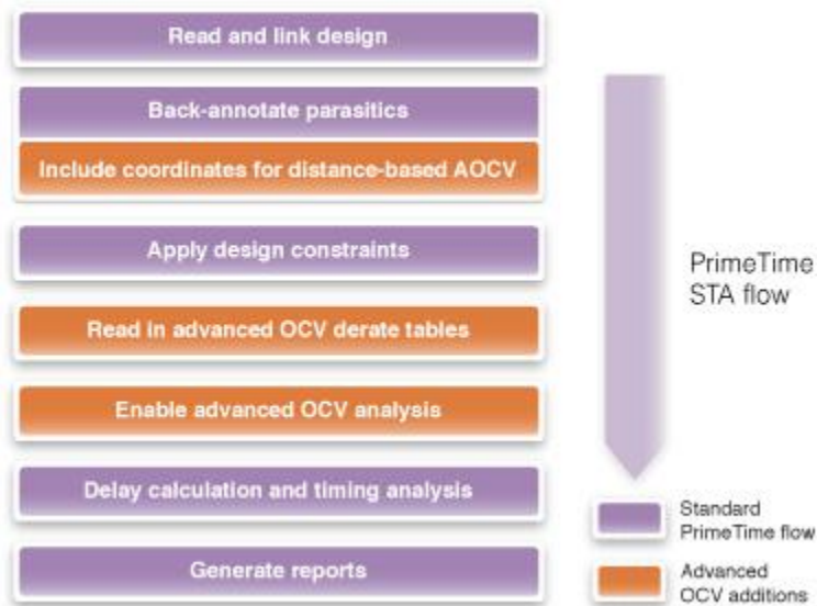
Figure 3: Minimal Script Edits Needed for Advanced OCV
